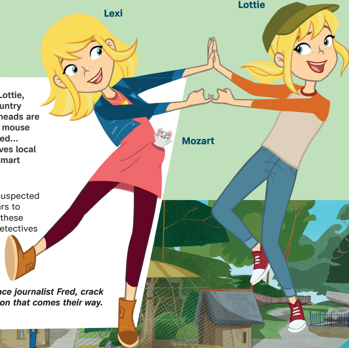
Lottie
